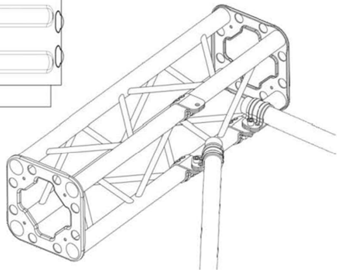
Two-piece fittings for easily connecting the pipes to the structure body allowing for different applications
