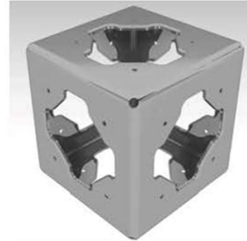
Cubic connectors for vertical attachment of modules
